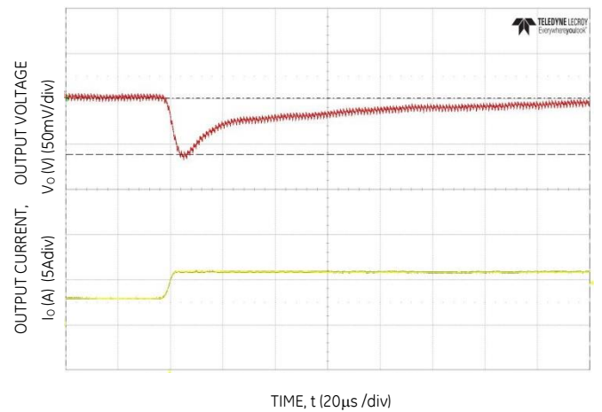
Figure 28. Transient Response to Dynamic Load Change from 50% to 100% at 12Vin, C_{out}=5 \times 47 \mu\text{F} , C_{Tune}=1800\text{pF} , R_{Tune}=300
